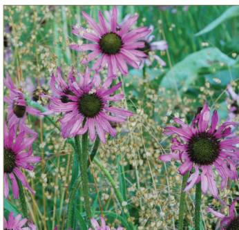
Echinacea tenesseeensis
