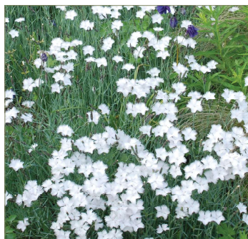
Dianthus 'Greystone'
